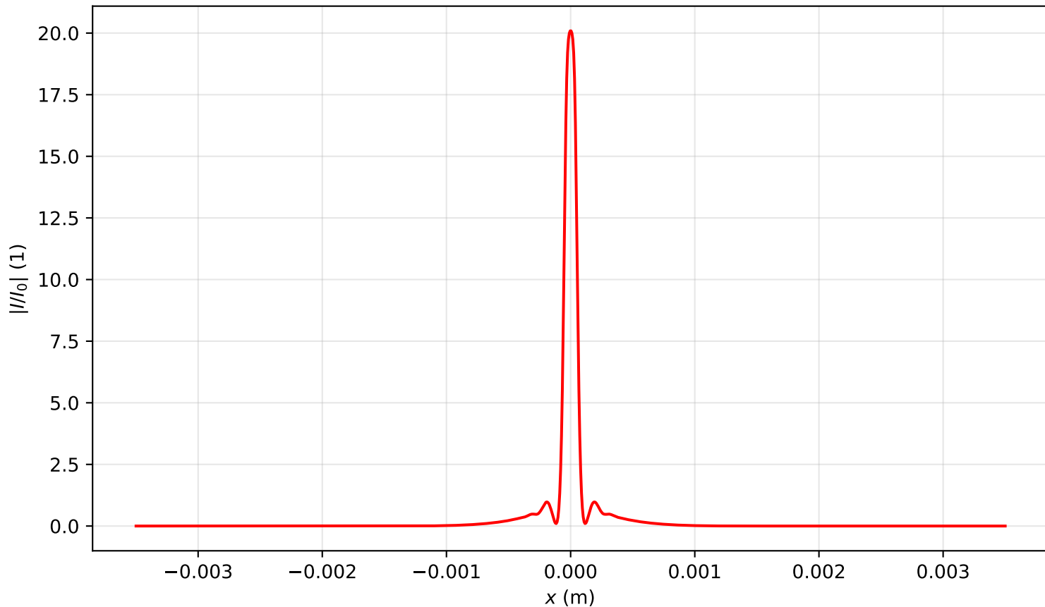
Intensity profile I(x, y = 0, z = 0.478)/I_0 , P_{in}=5.5P_{cr} , artificial time
